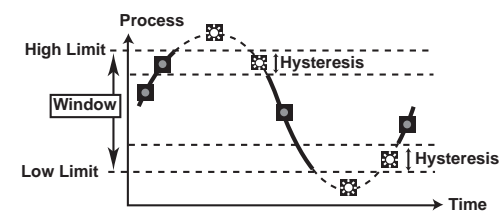
Relay behavior with WINDOW Setpoints
